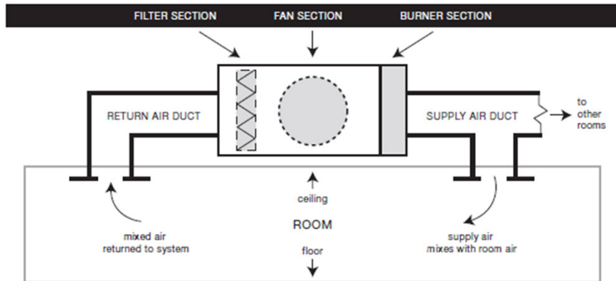
Recirculating Central Ventilation Unit
