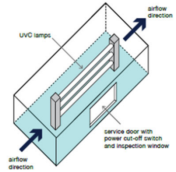
FIGURE 5. Schematic of in-duct UVC 254 system
